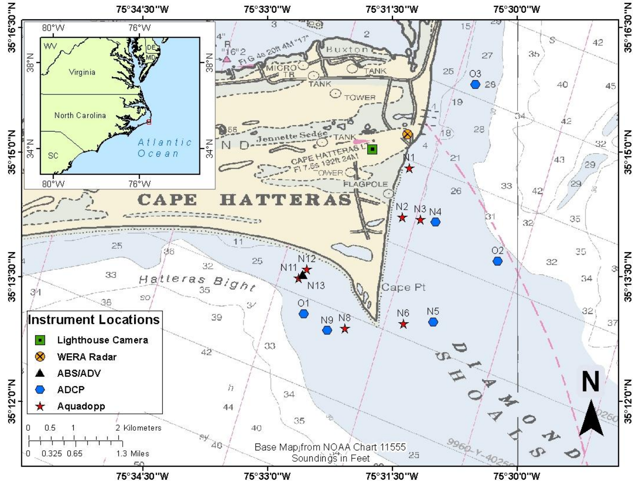
Figure 1. Location map for Cape Hatteras, North Carolina. Markers are placed to identify the nearshore (starting with “N”), offshore (starting with “O”), lighthouse, and Wellen radar (WERA) sites. Locations for Aquadopps (current profiler utilizing Doppler technology), acoustic backscatter sensor (ABS), acoustic Doppler velocimeter (ADV), and acoustic Doppler current profilers (ADCP) are identified.
